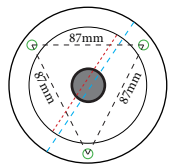
Wall mount base, back
